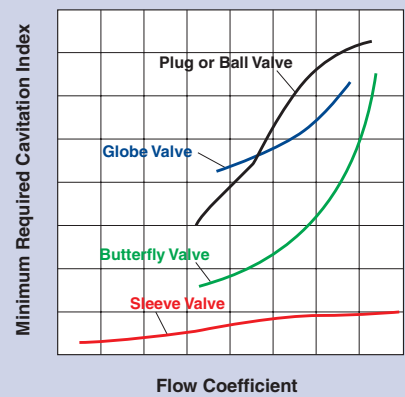
Cavitation Index Curve
